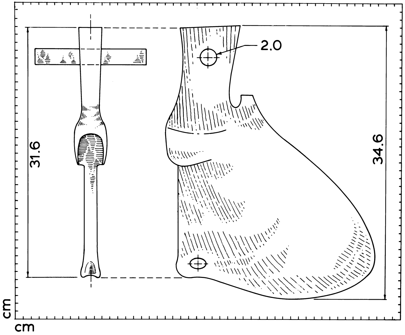
RUDDER
