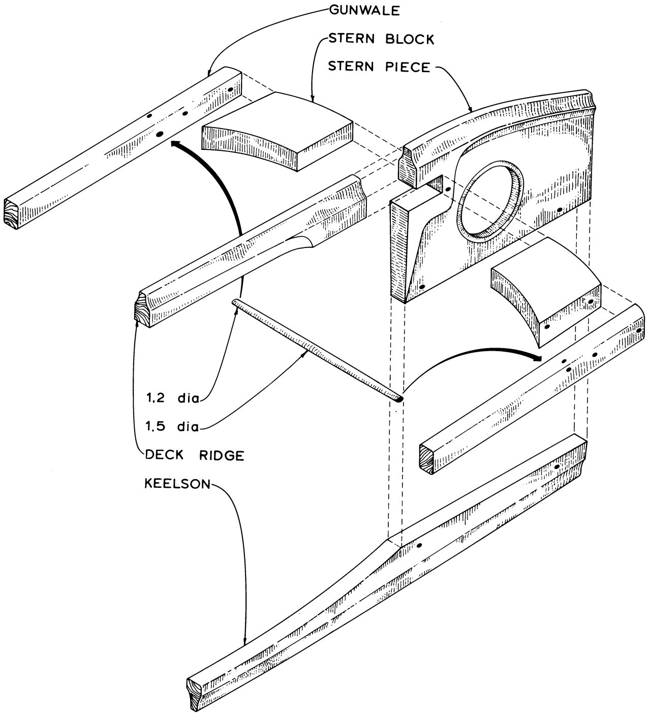
STERN CONSTRUCTION
