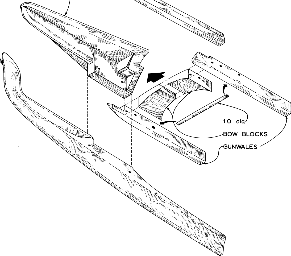
BOW CONSTRUCTION
