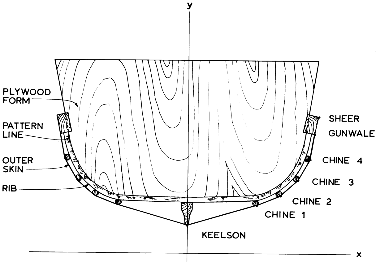
STATION 6
